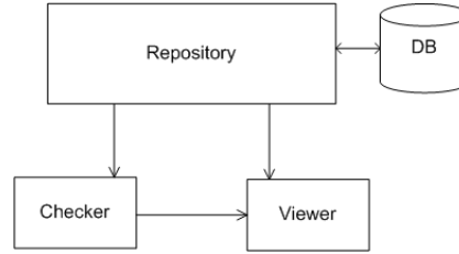
Fig. 5. Component model
